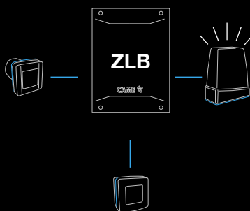
STAR connection
